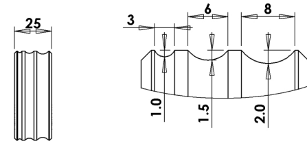
Extension Roll No2
