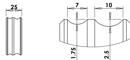
Extension Roll No3
