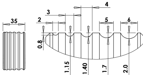
Extension Roll No1
